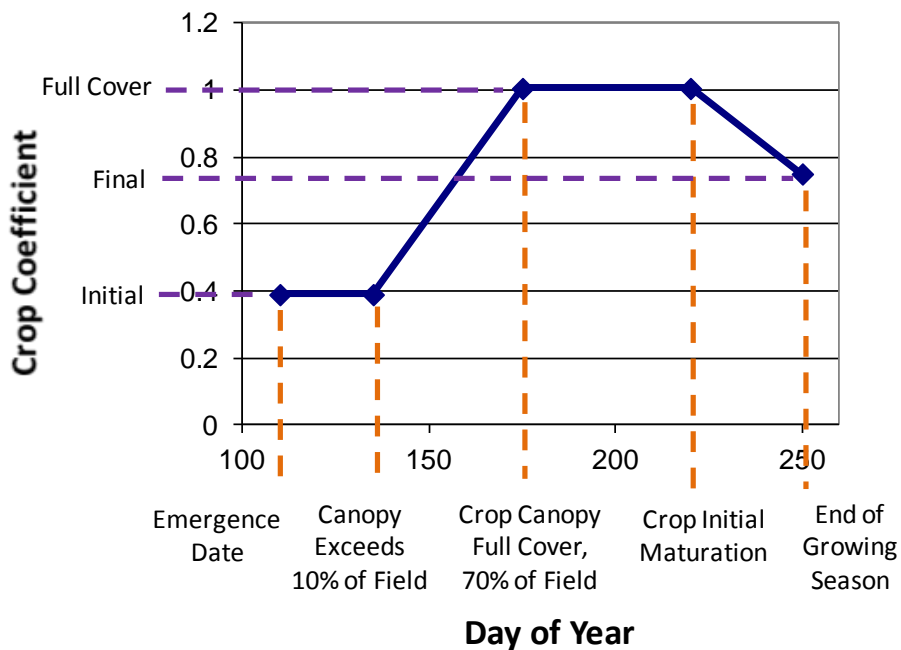
Figure 7. Parameters that define the crop coefficient curve. The crop coefficient is multiplied by the alfalfa reference ET rate to determine the crop water use for that day. Defaults values for these parameters are set based on the crop chosen, but can be modified in “Advanced Field Settings.”
